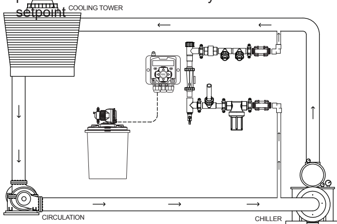
Typical Cooling Tower Installation
